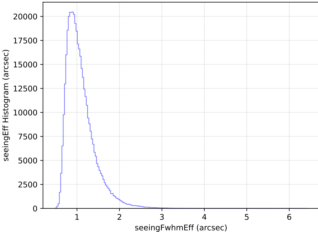
internal_u_expt45_nscale1.2v3.4_10yrs All sky z band: seeingEff Histogram
