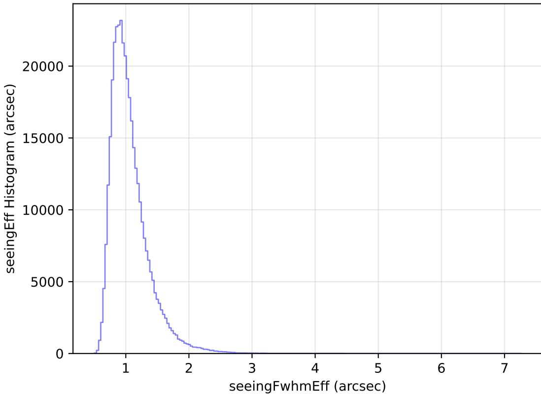
internal_u_expt45_nscale1.2v3.4_10yrs All sky y band: seeingEff Histogram
