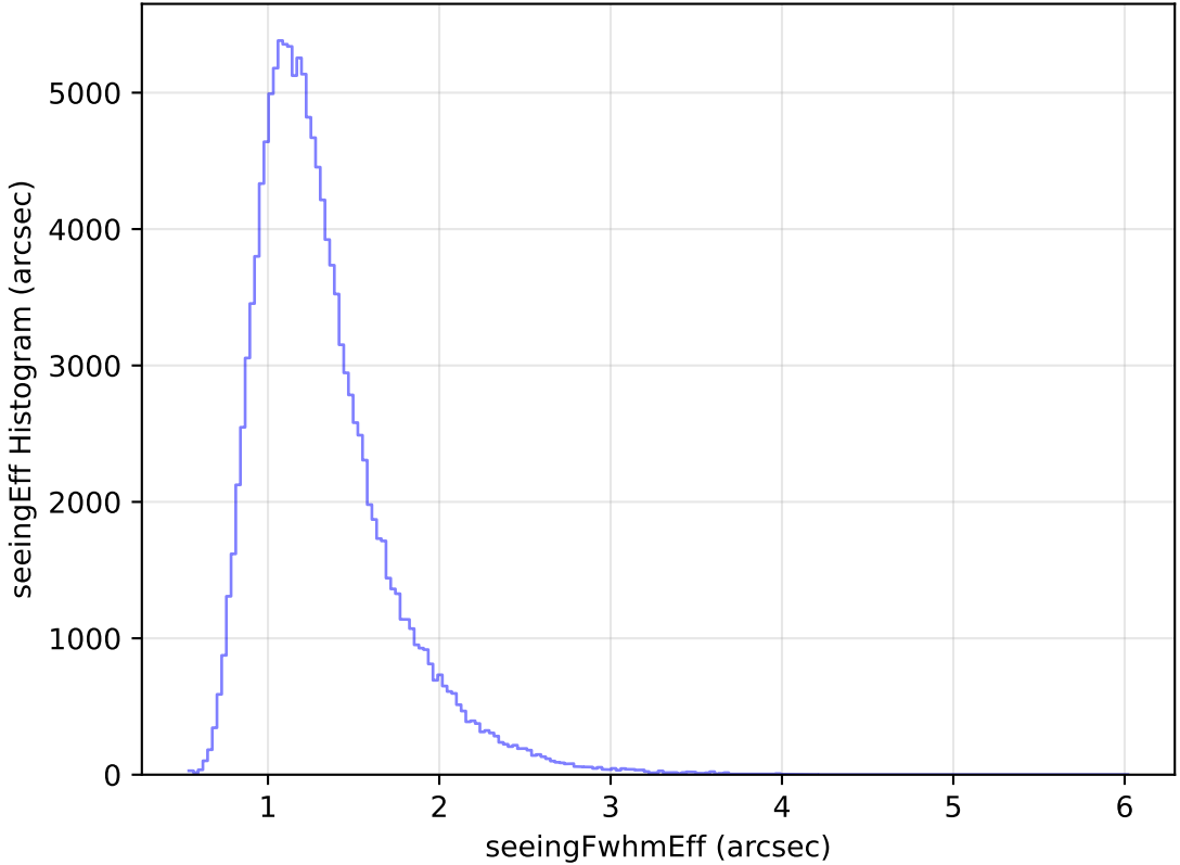
internal_u_expt45_nscale1.2v3.4_10yrs All sky u band: seeingEff Histogram
