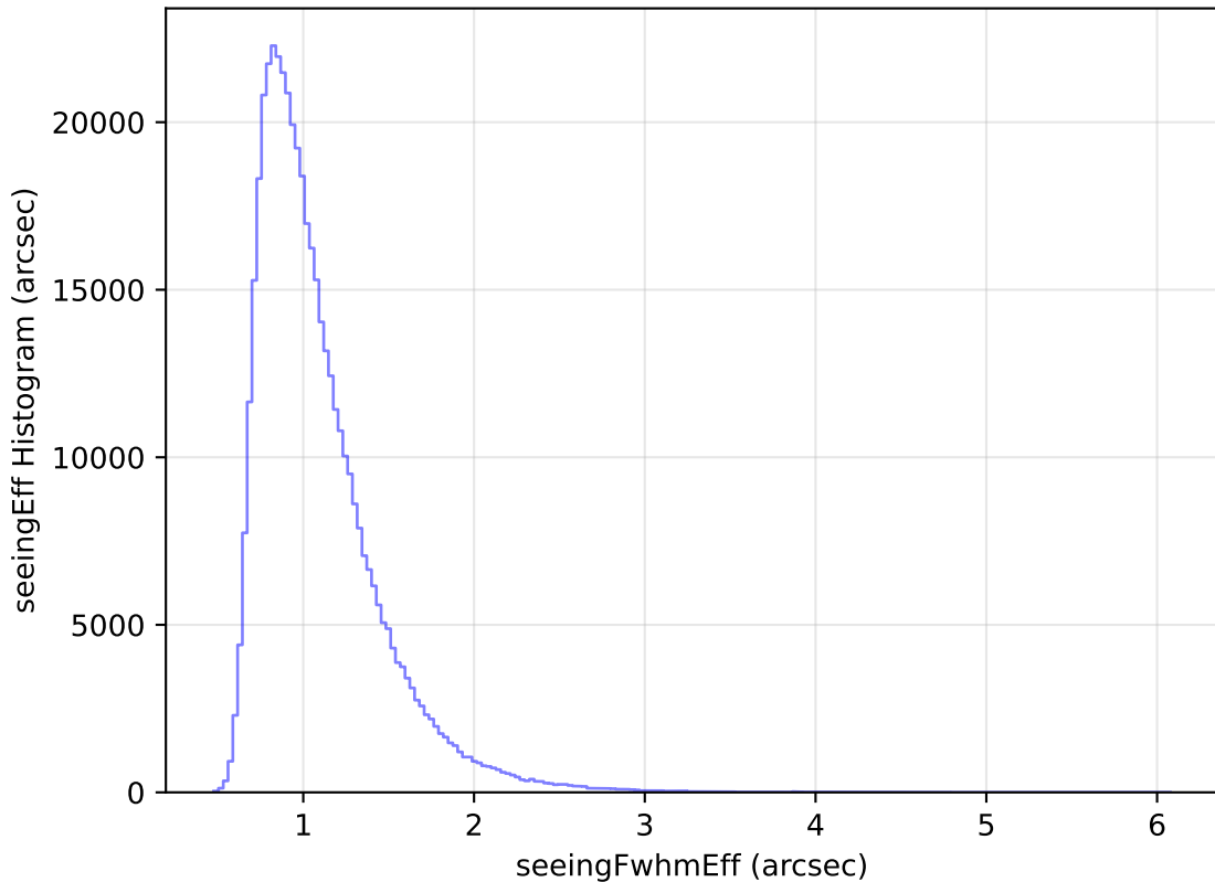
internal_u_expt45_nscale1.2v3.4_10yrs All sky i band: seeingEff Histogram
