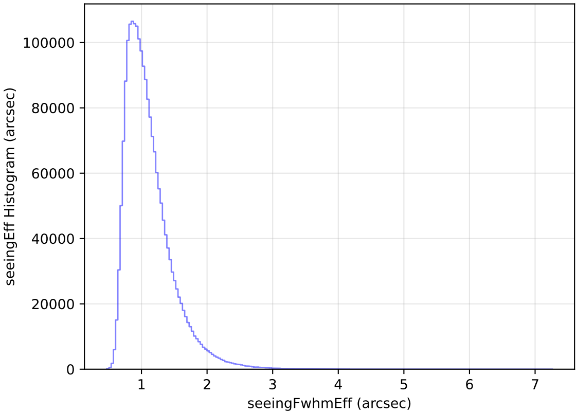
internal_u_expt45_nscale1.2v3.4_10yrs All sky all bands: seeingEff Histogram
