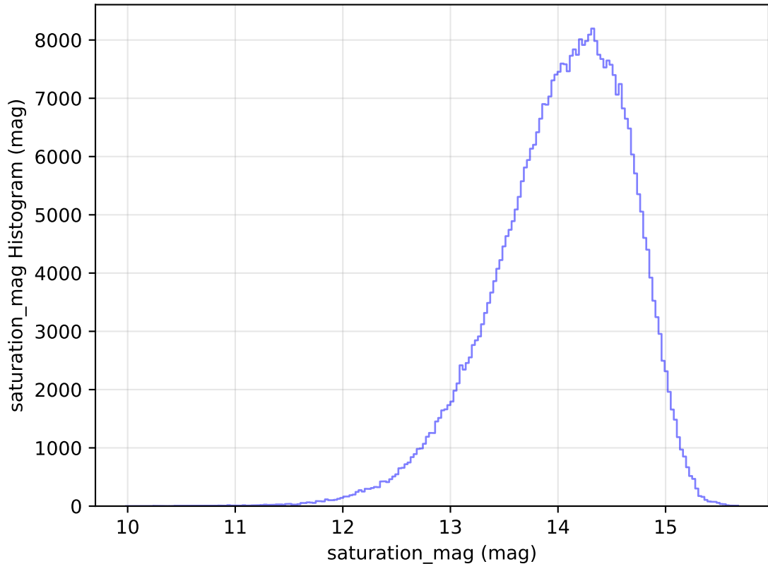
internal_u_expt45_nscale1.2v3.4_10yrs WFD z band: saturation_mag Histogram
