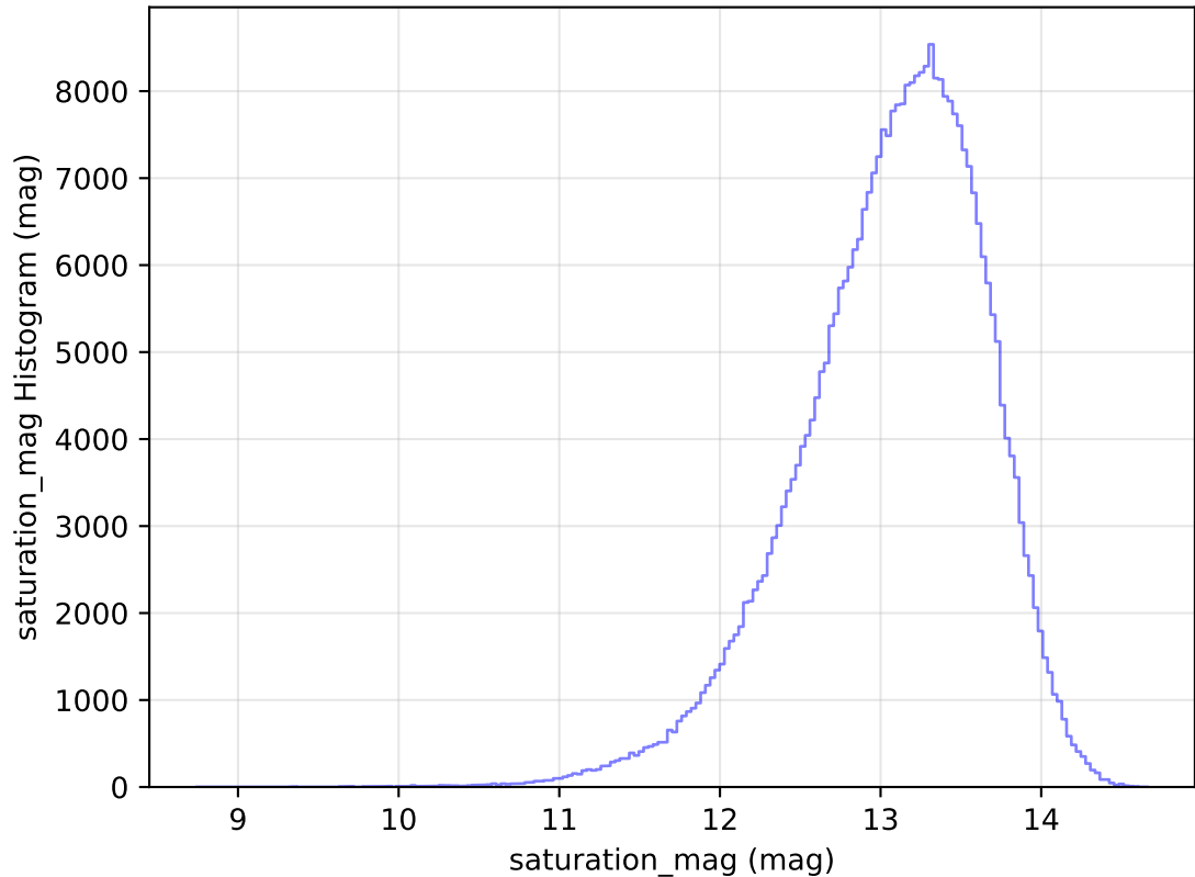
internal_u_expt45_nscale1.2v3.4_10yrs WFD y band: saturation_mag Histogram
