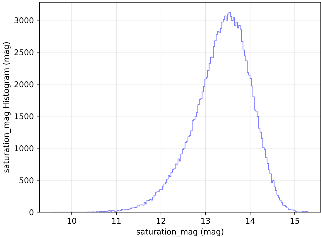
internal_u_expt45_nscale1.2v3.4_10yrs WFD u band: saturation_mag Histogram
