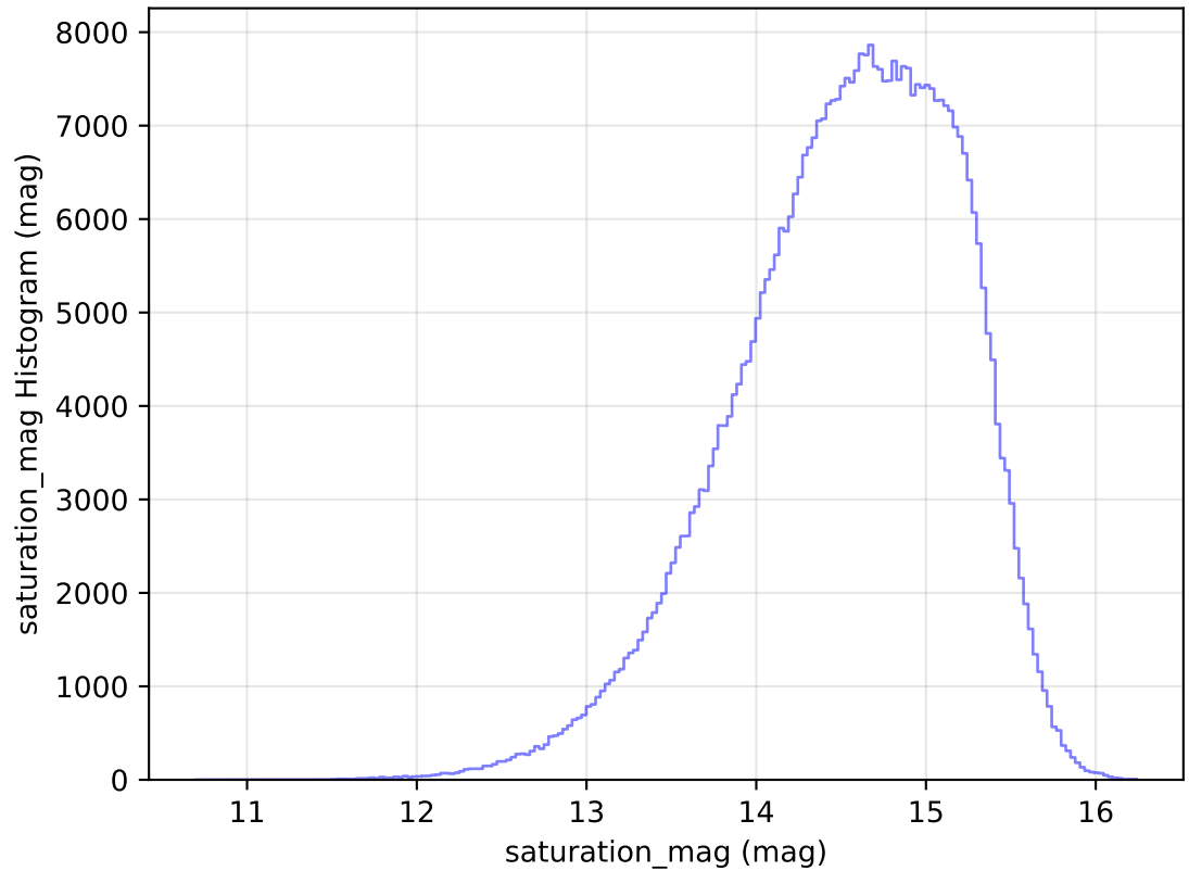
internal_u_expt45_nscale1.2v3.4_10yrs WFD r band: saturation_mag Histogram
