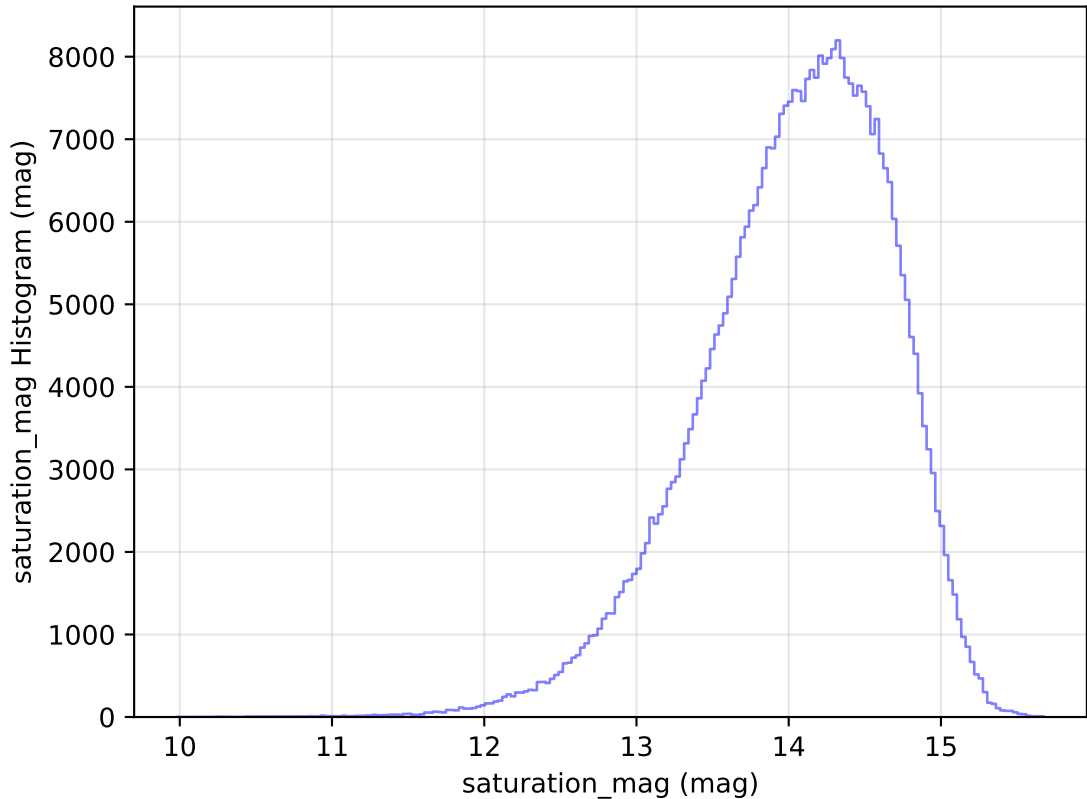
internal_u_expt45_nscale1.2v3.4_10yrs All sky z band: saturation_mag Histogram
