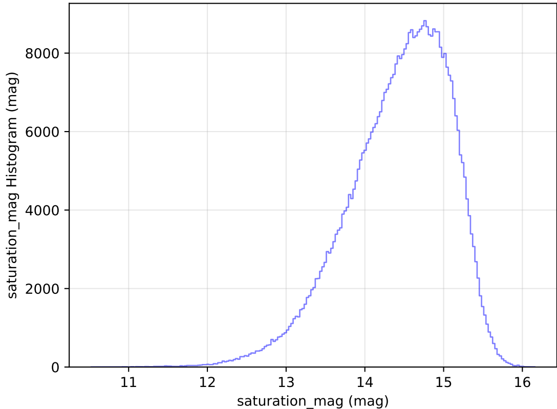
internal_u_expt45_nscale1.2v3.4_10yrs All sky i band: saturation_mag Histogram
