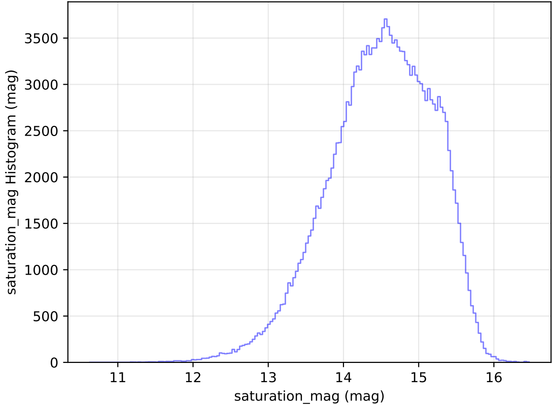
internal_u_expt45_nscale1.2v3.4_10yrs All sky g band: saturation_mag Histogram
