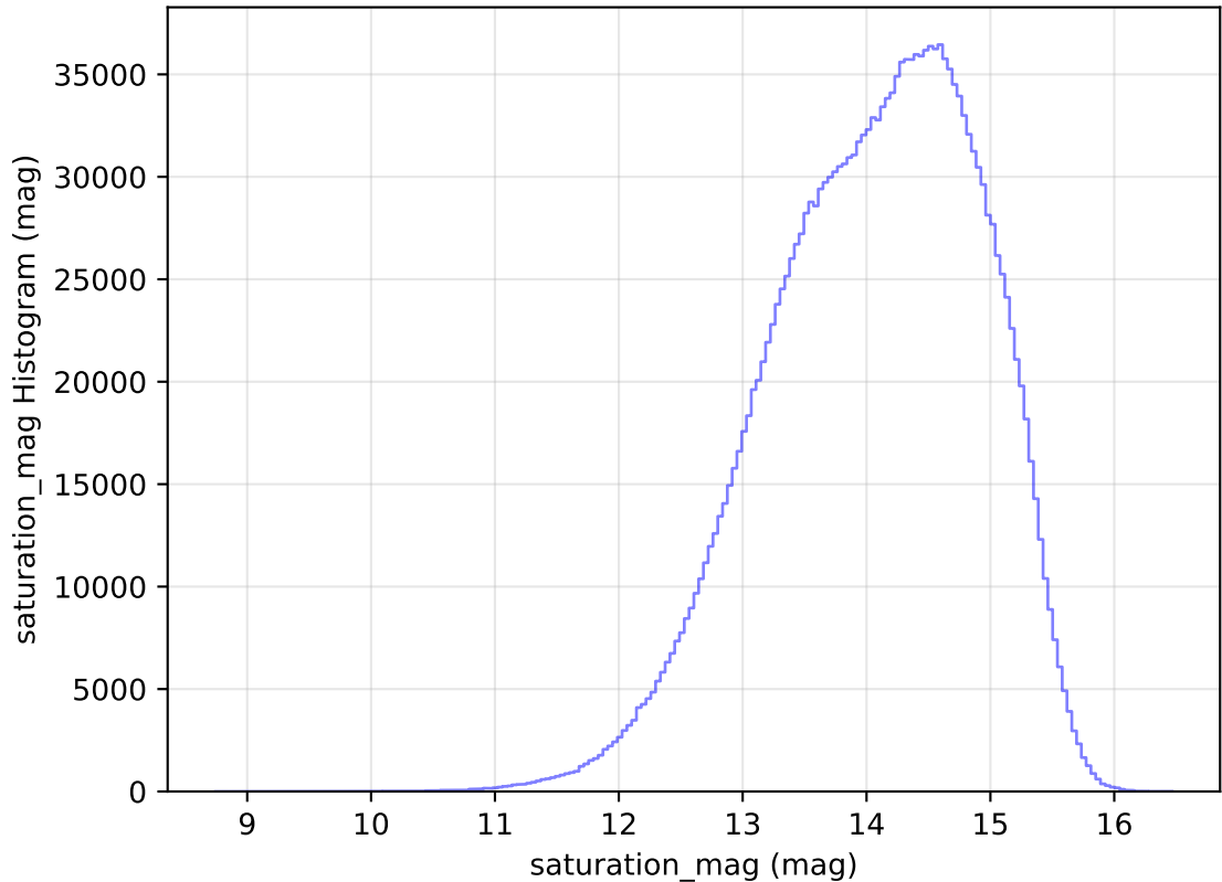
internal_u_expt45_nscale1.2v3.4_10yrs All sky all bands: saturation_mag Histogram
