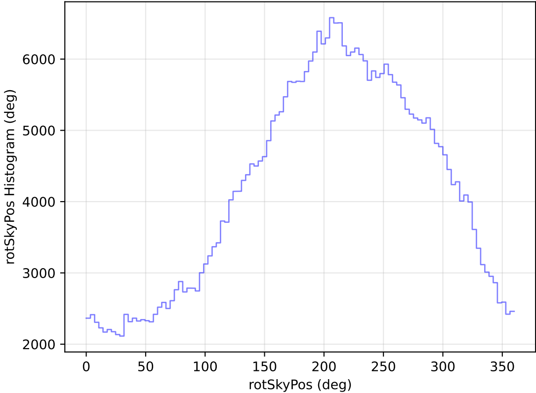
internal_u_expt45_nscale1.2v3.4_10yrs WFD z band: rotSkyPos Histogram
