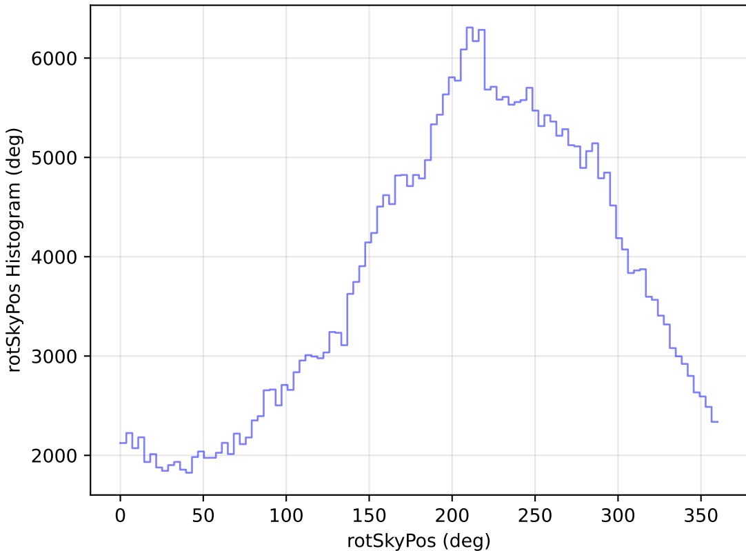
internal_u_expt45_nscale1.2v3.4_10yrs WFD y band: rotSkyPos Histogram
