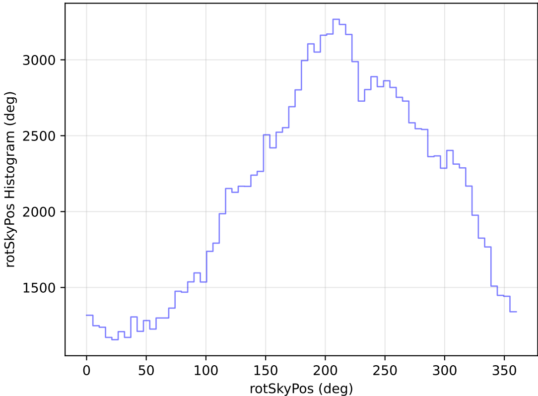
internal_u_expt45_nscale1.2v3.4_10yrs WFD u band: rotSkyPos Histogram
