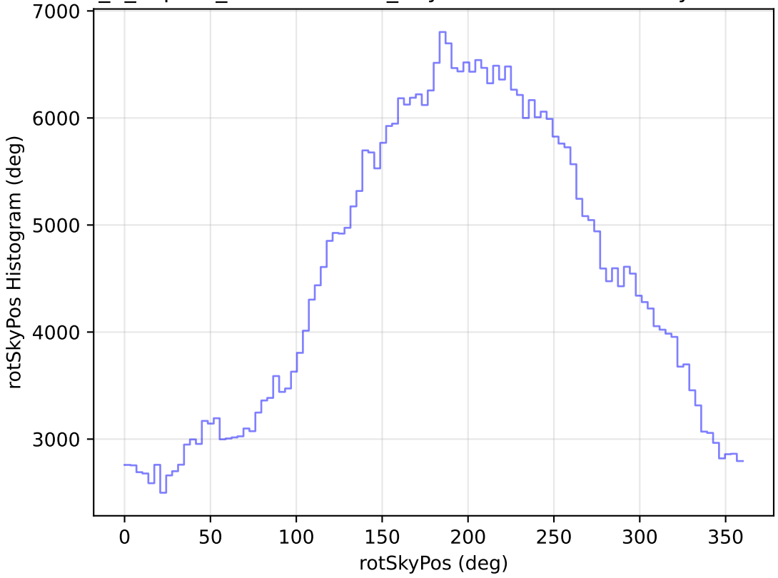
internal_u_expt45_nscale1.2v3.4_10yrs WFD r band: rotSkyPos Histogram
