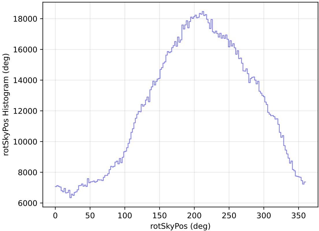
internal_u_expt45_nscale1.2v3.4_10yrs WFD all bands: rotSkyPos Histogram
