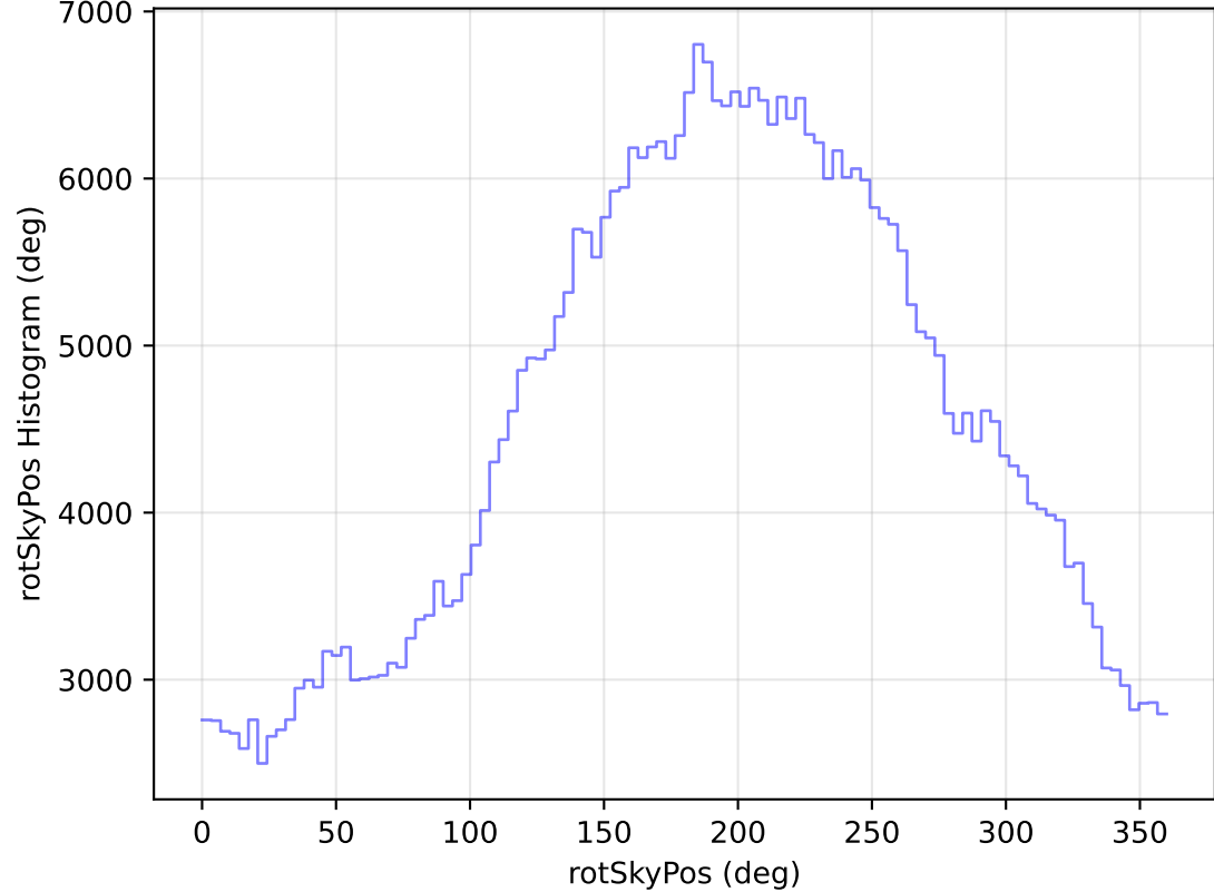
internal_u_expt45_nscale1.2v3.4_10yrs All sky r band: rotSkyPos Histogram
