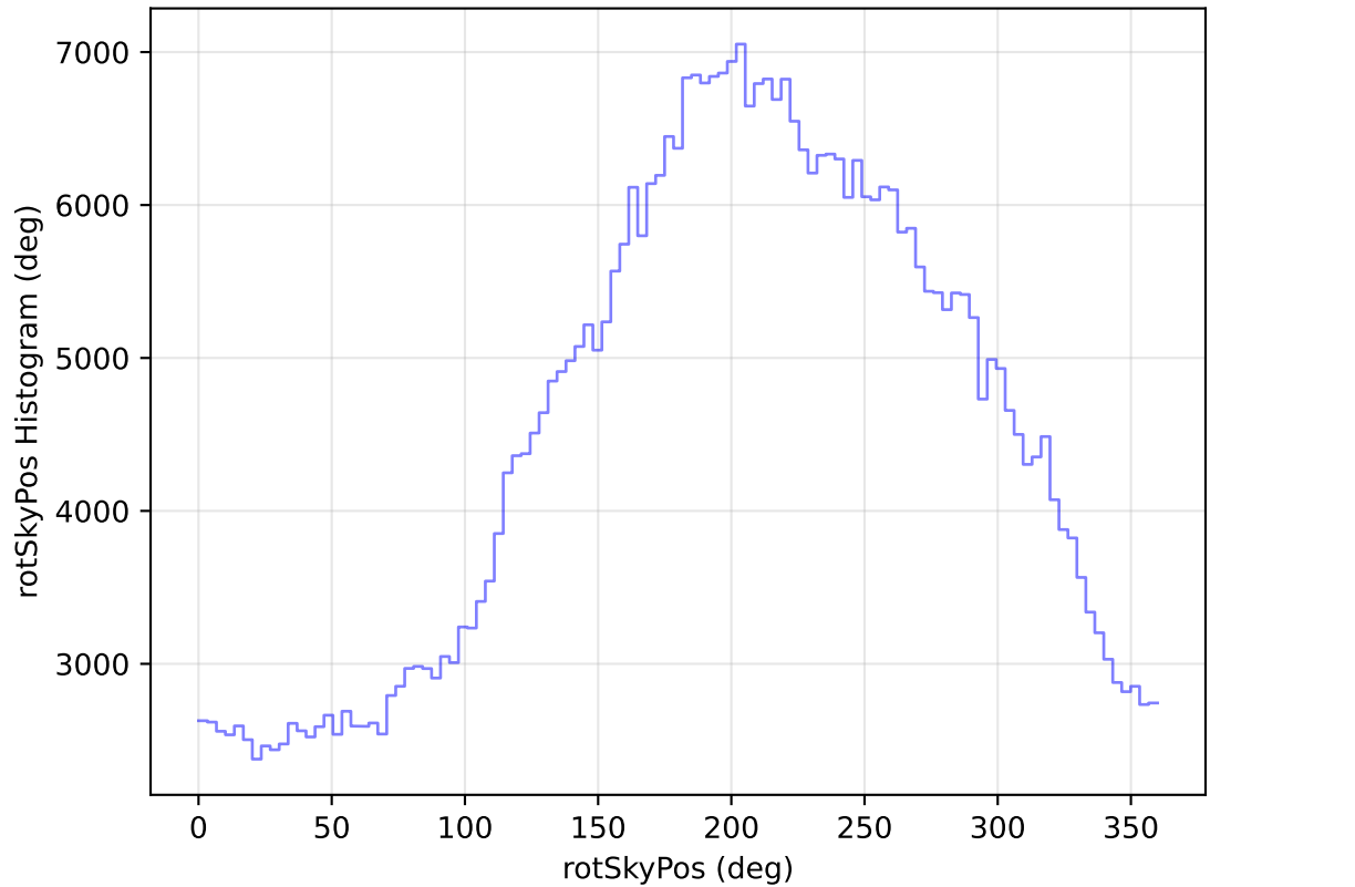
internal_u_expt45_nscale1.2v3.4_10yrs All sky i band: rotSkyPos Histogram
