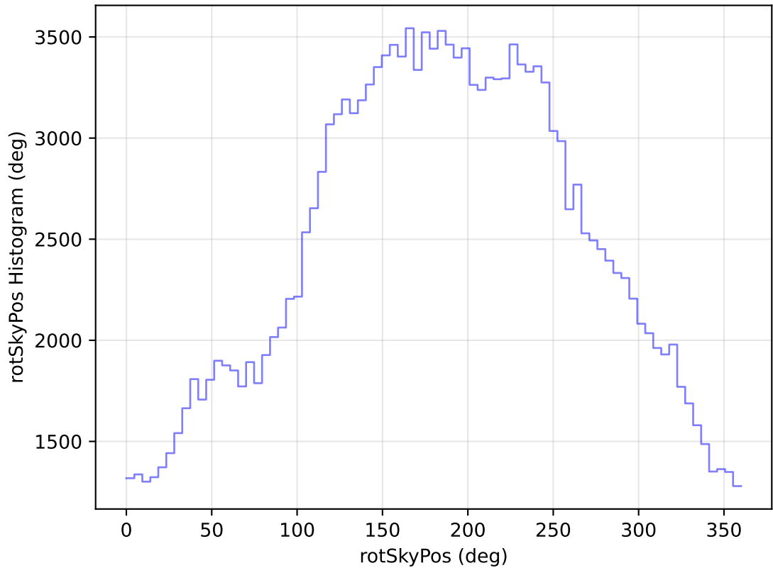
internal_u_expt45_nscale1.2v3.4_10yrs All sky g band: rotSkyPos Histogram
