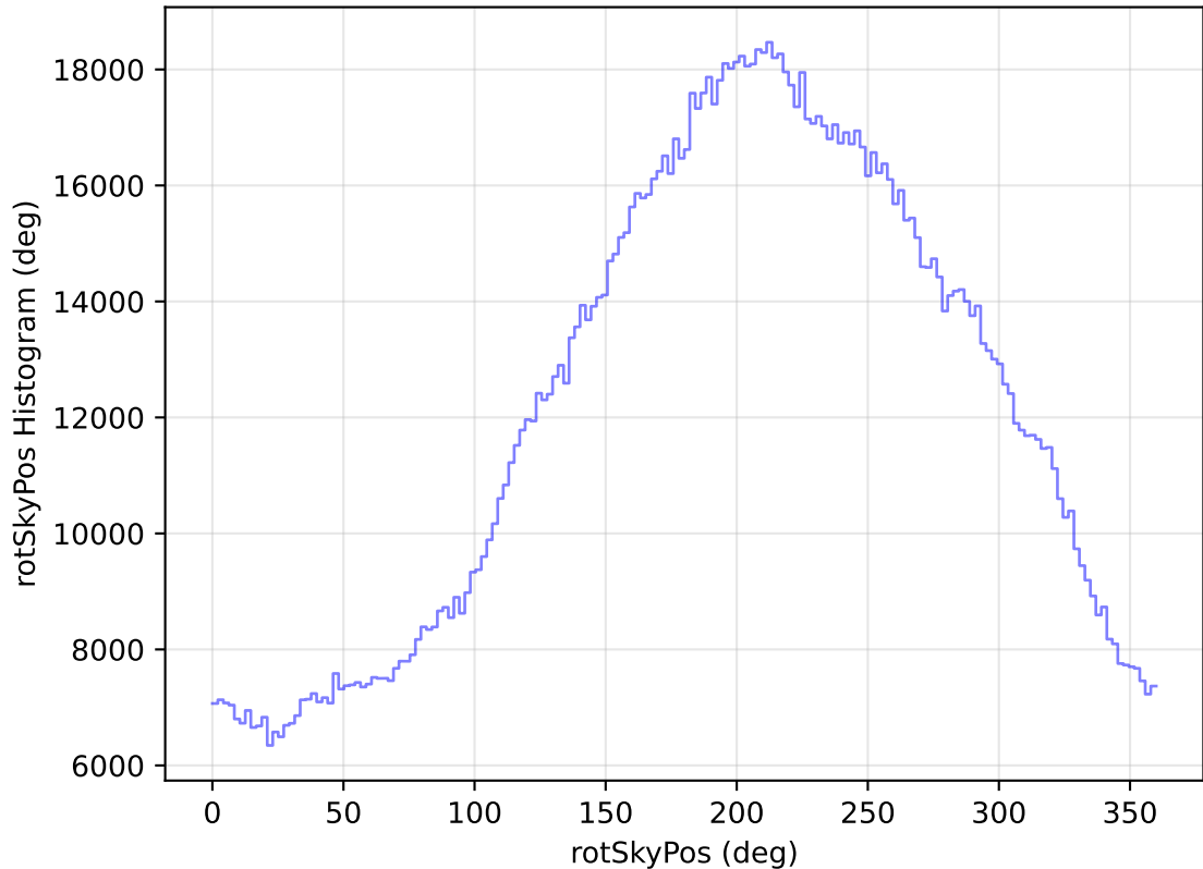
internal_u_expt45_nscale1.2v3.4_10yrs All sky all bands: rotSkyPos Histogram
