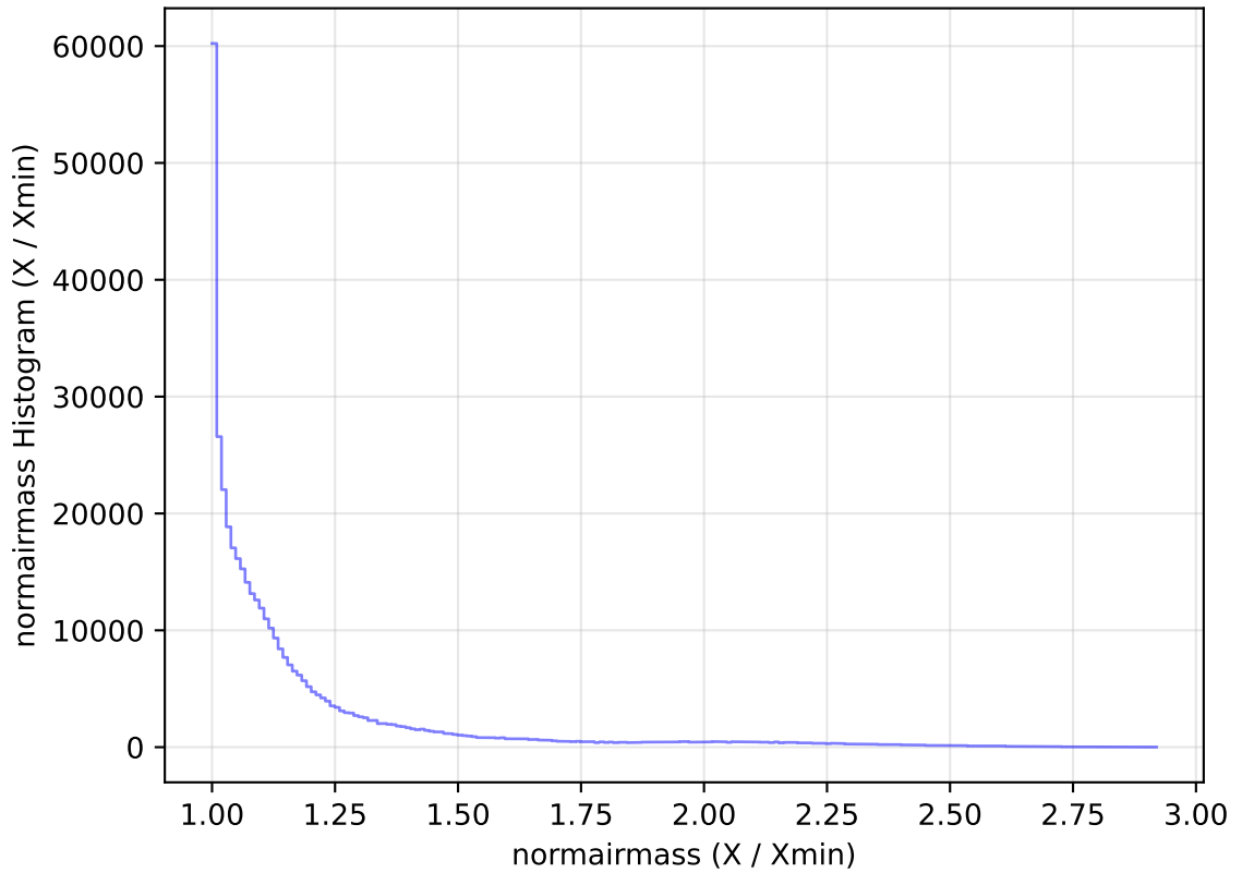
internal_u_expt45_nscale1.2v3.4_10yrs WFD z band: normairmass Histogram
