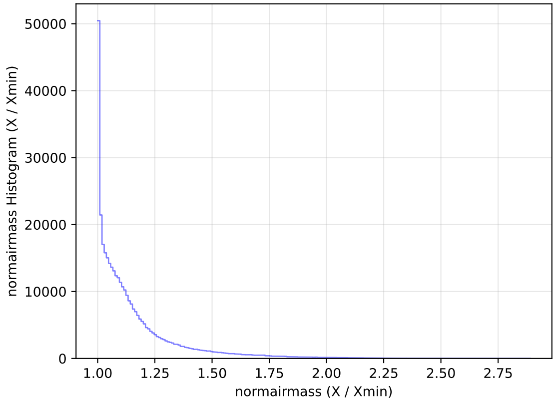
internal_u_expt45_nscale1.2v3.4_10yrs WFD y band: normairmass Histogram
