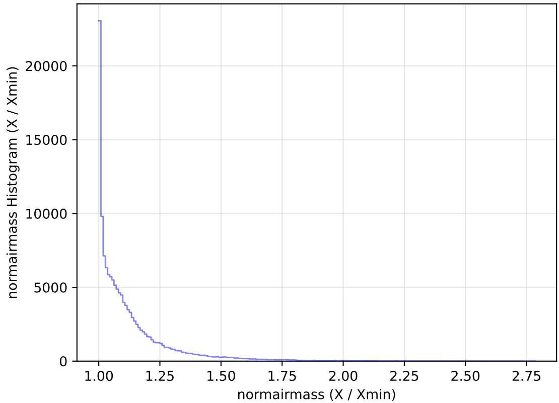
internal_u_expt45_nscale1.2v3.4_10yrs WFD u band: normairmass Histogram
