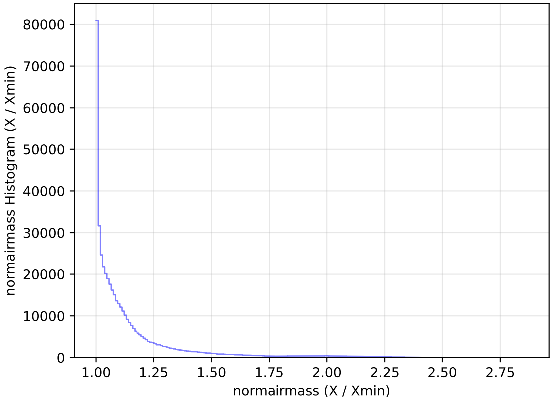
internal_u_expt45_nscale1.2v3.4_10yrs WFD r band: normairmass Histogram
