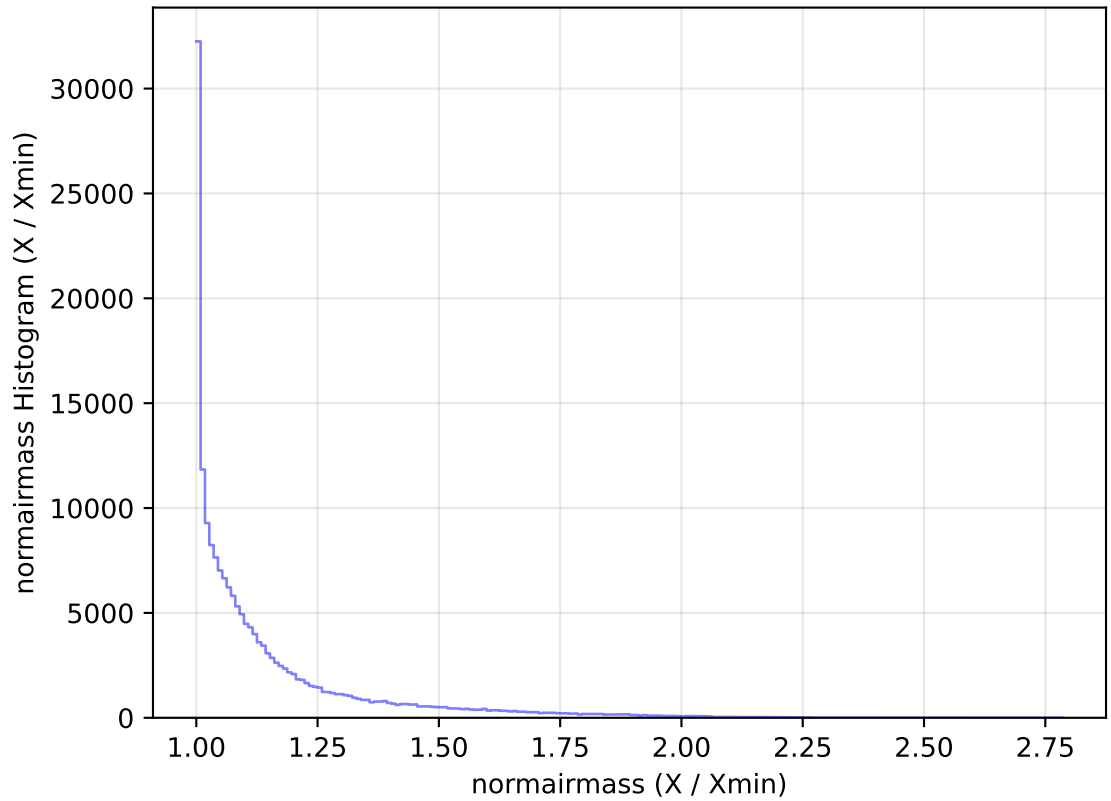
internal_u_expt45_nscale1.2v3.4_10yrs WFD g band: normairmass Histogram
