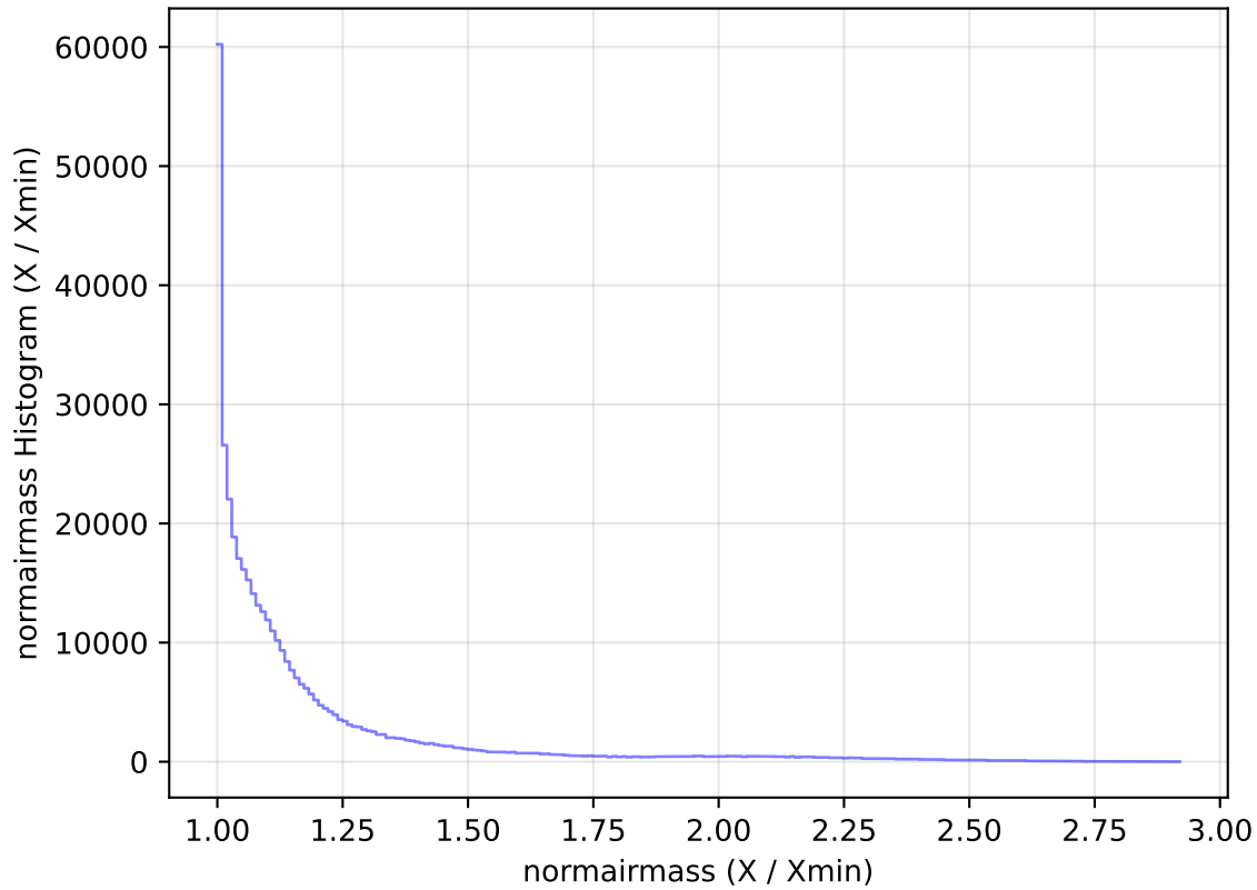
internal_u_expt45_nscale1.2v3.4_10yrs All sky z band: normairmass Histogram
