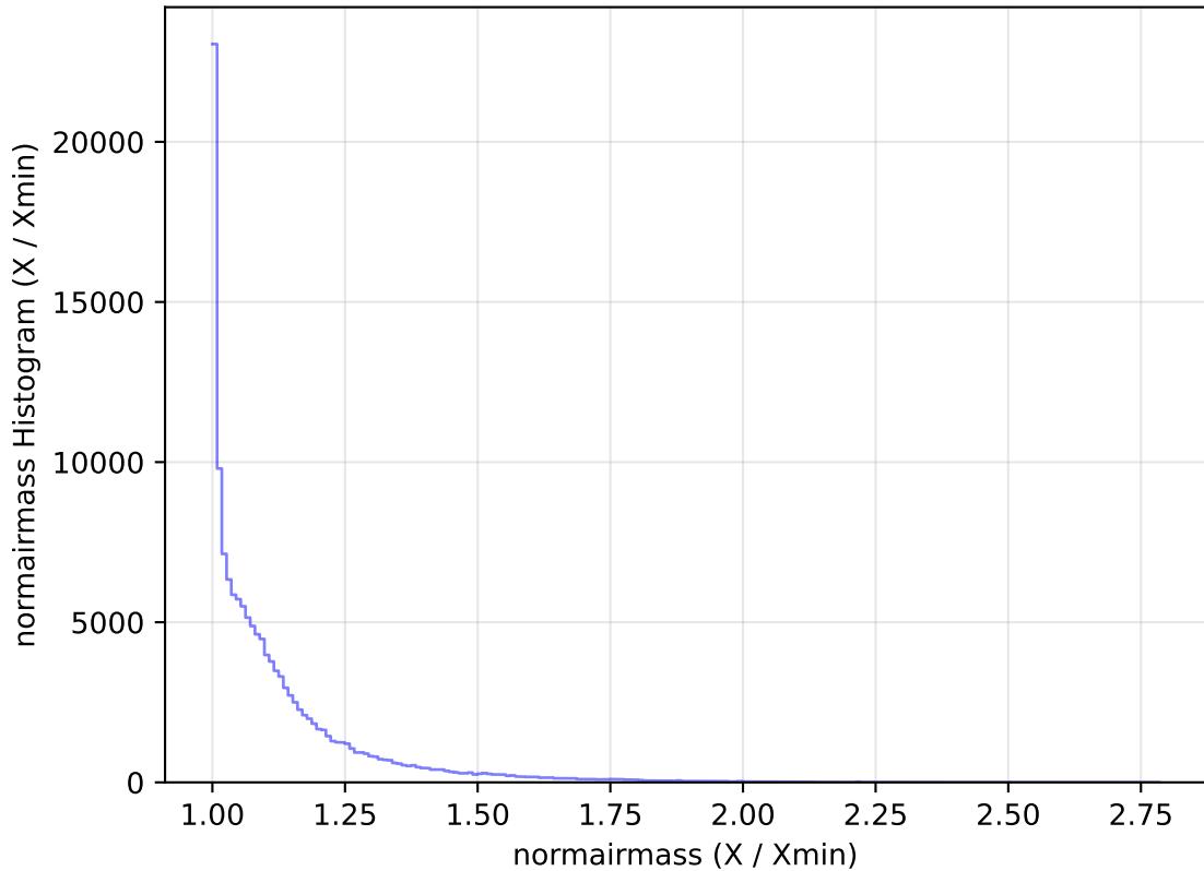
internal_u_expt45_nscale1.2v3.4_10yrs All sky u band: normairmass Histogram
