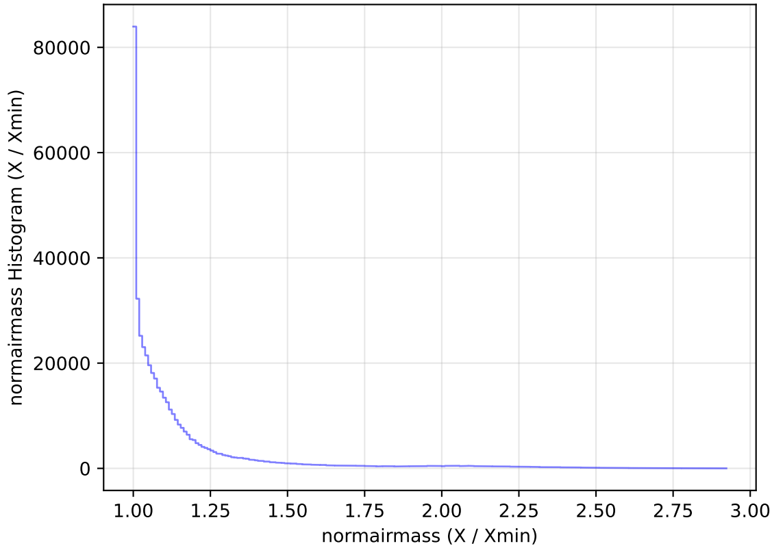
internal_u_expt45_nscale1.2v3.4_10yrs All sky i band: normairmass Histogram
