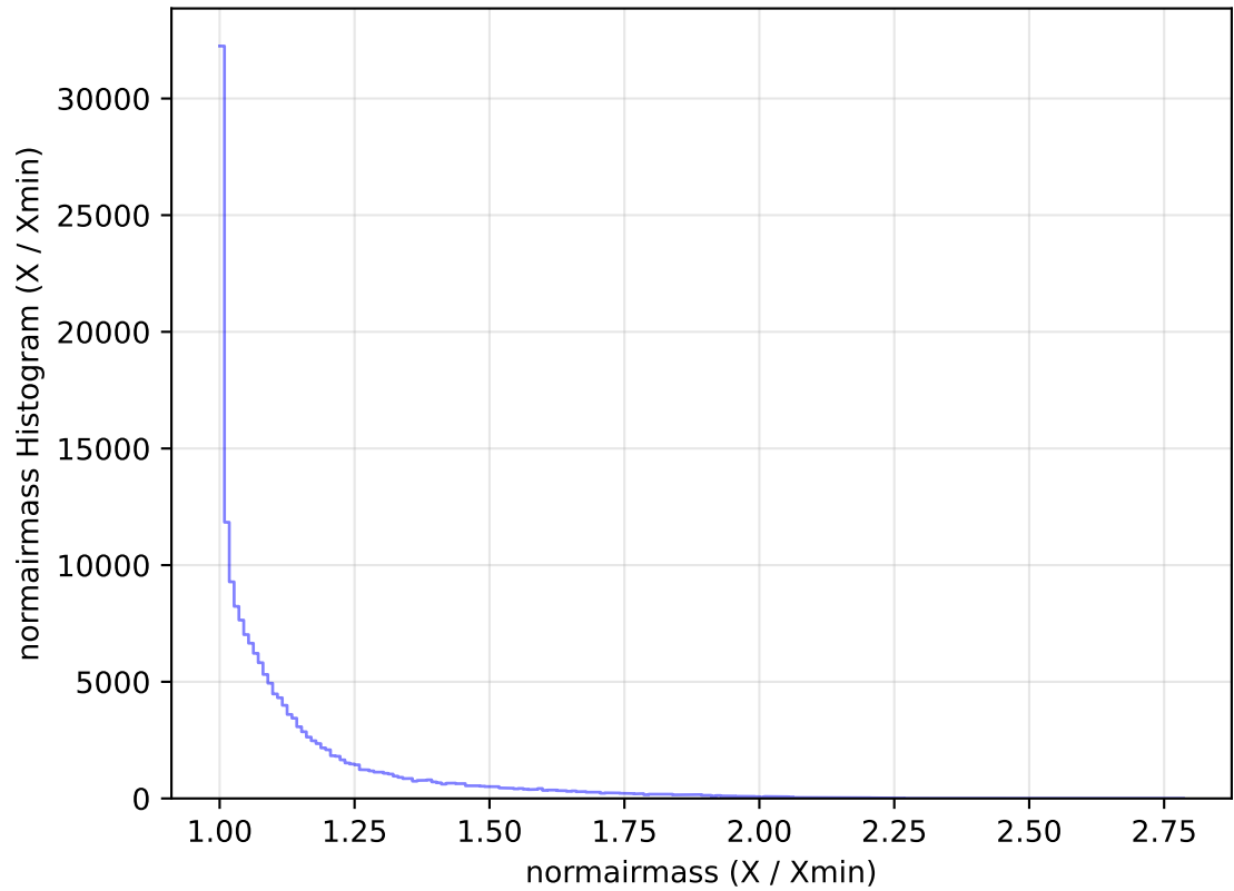
internal_u_expt45_nscale1.2v3.4_10yrs All sky g band: normairmass Histogram
