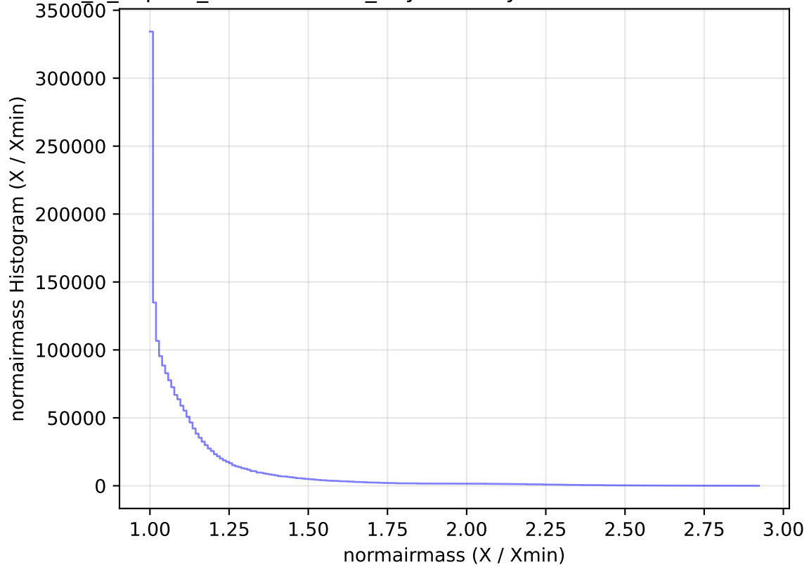
internal_u_expt45_nscale1.2v3.4_10yrs All sky all bands: normairmass Histogram
