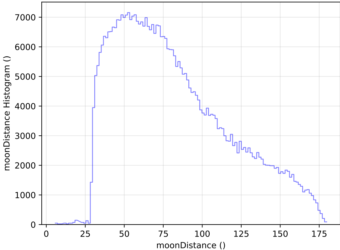
internal_u_expt45_nscale1.2v3.4_10yrs WFD z band: moonDistance Histogram
