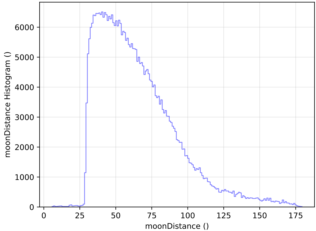
internal_u_expt45_nscale1.2v3.4_10yrs WFD y band: moonDistance Histogram
