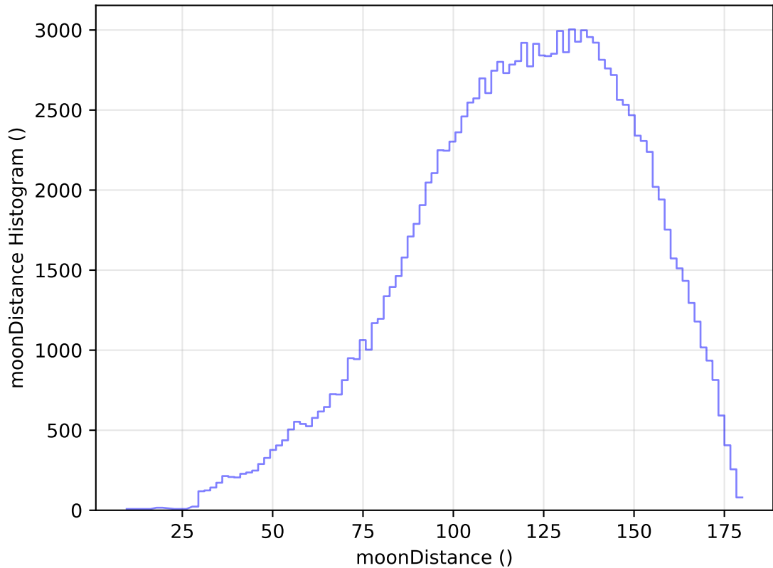
internal_u_expt45_nscale1.2v3.4_10yrs WFD u band: moonDistance Histogram
