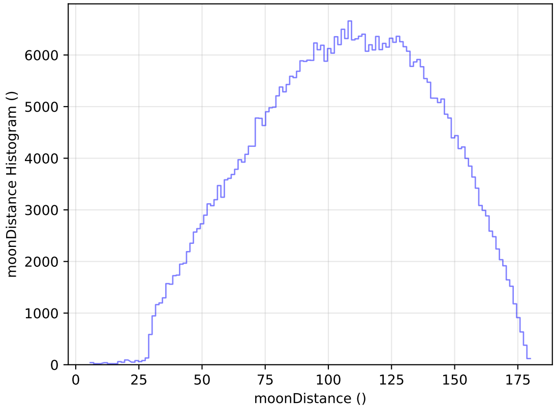
internal_u_expt45_nscale1.2v3.4_10yrs WFD r band: moonDistance Histogram
