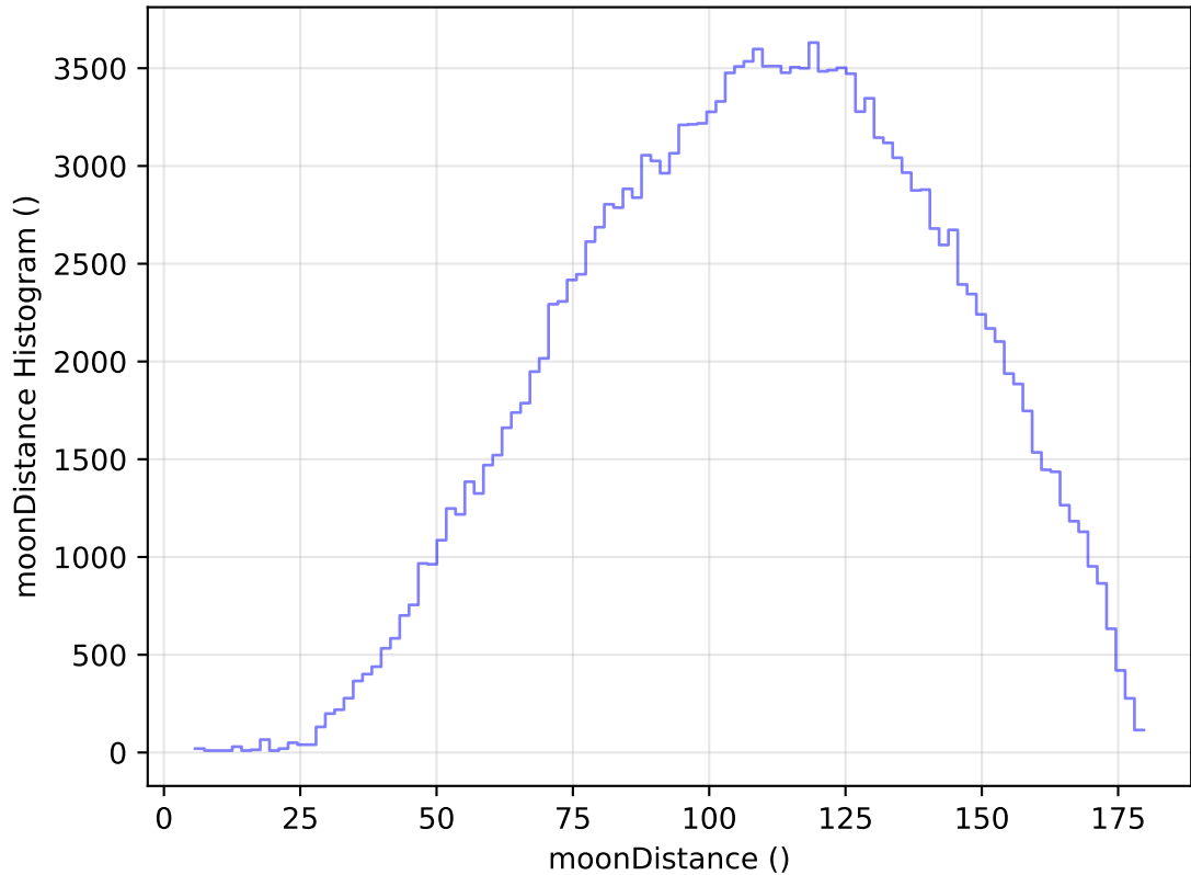
internal_u_expt45_nscale1.2v3.4_10yrs WFD g band: moonDistance Histogram
