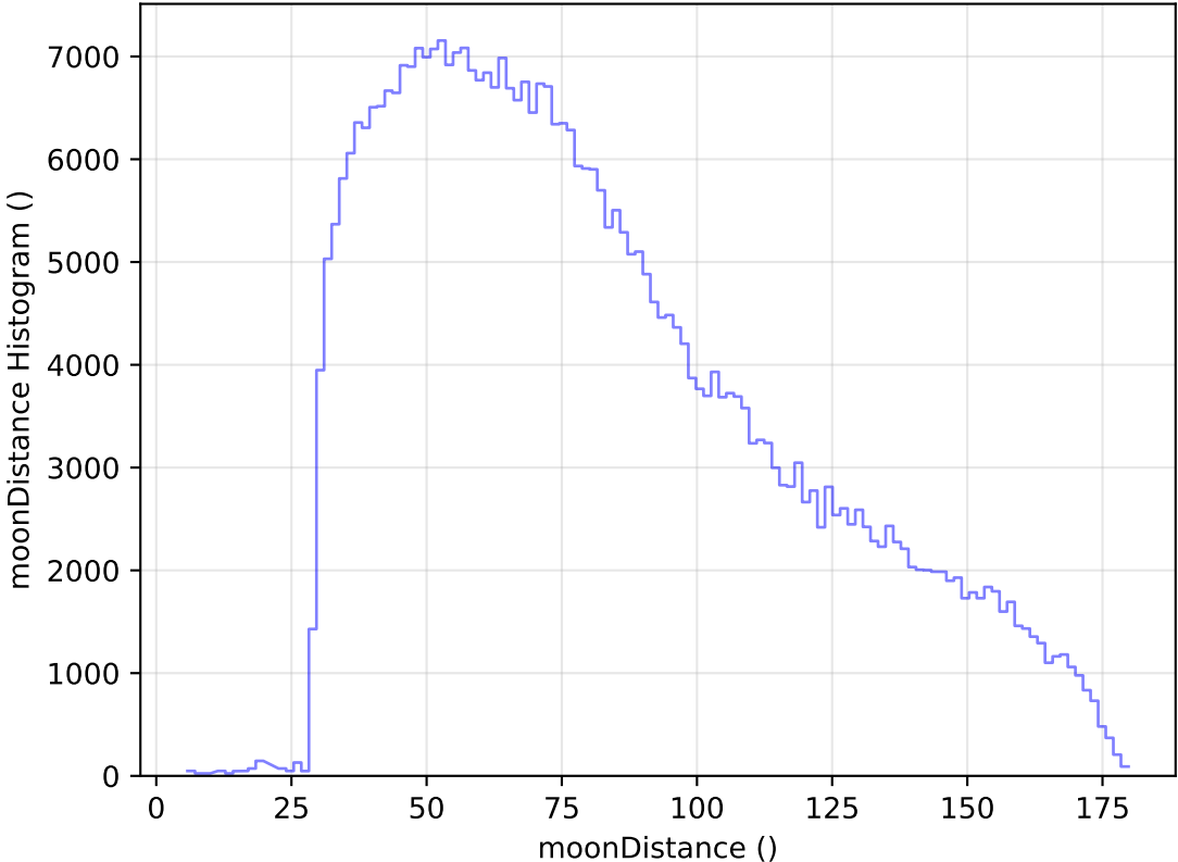
internal_u_expt45_nscale1.2v3.4_10yrs All sky z band: moonDistance Histogram
