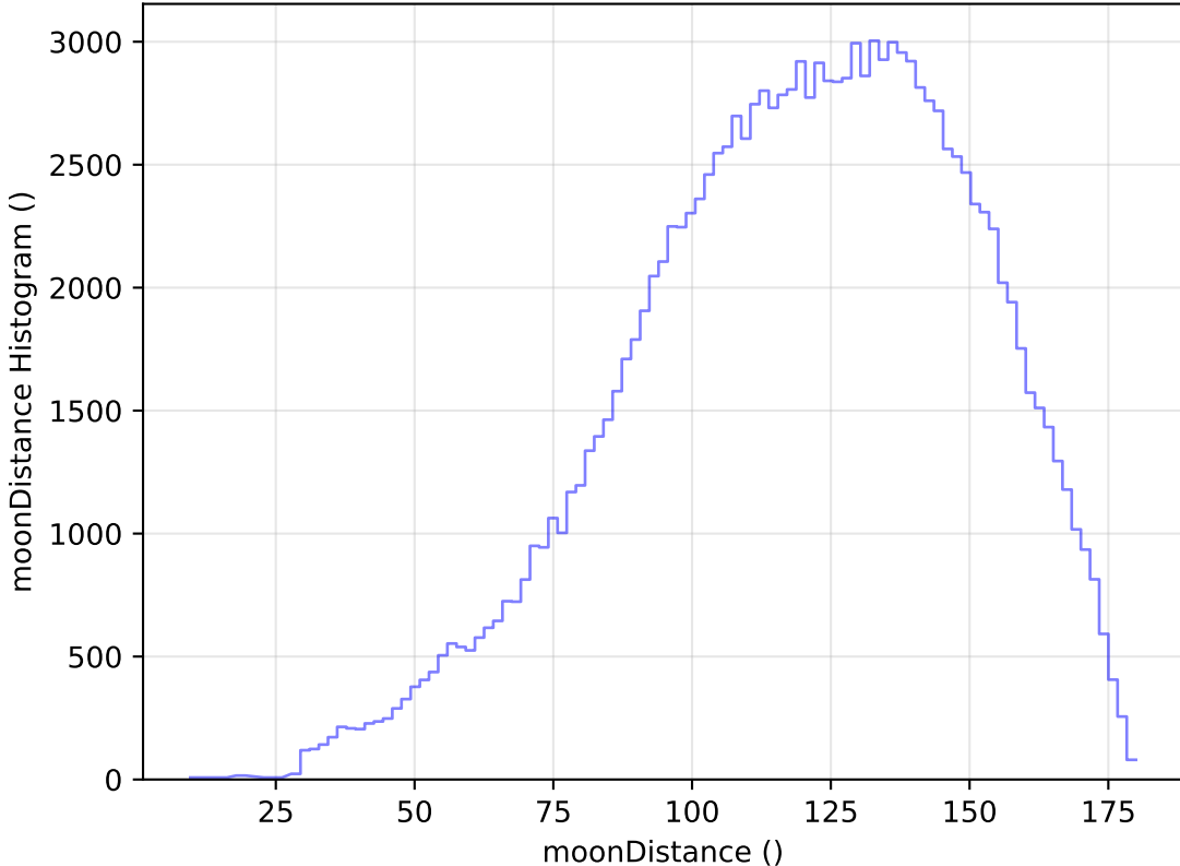
internal_u_expt45_nscale1.2v3.4_10yrs All sky u band: moonDistance Histogram
