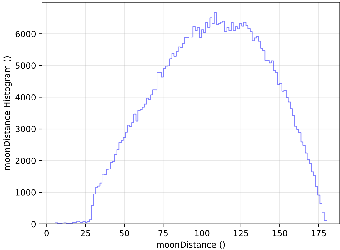
internal_u_expt45_nscale1.2v3.4_10yrs All sky r band: moonDistance Histogram
