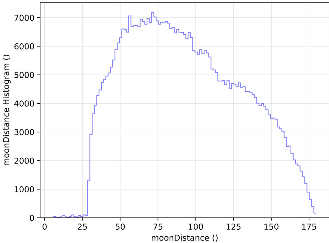
internal_u_expt45_nscale1.2v3.4_10yrs All sky i band: moonDistance Histogram
