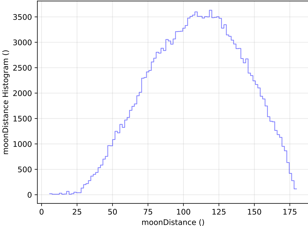
internal_u_expt45_nscale1.2v3.4_10yrs All sky g band: moonDistance Histogram
