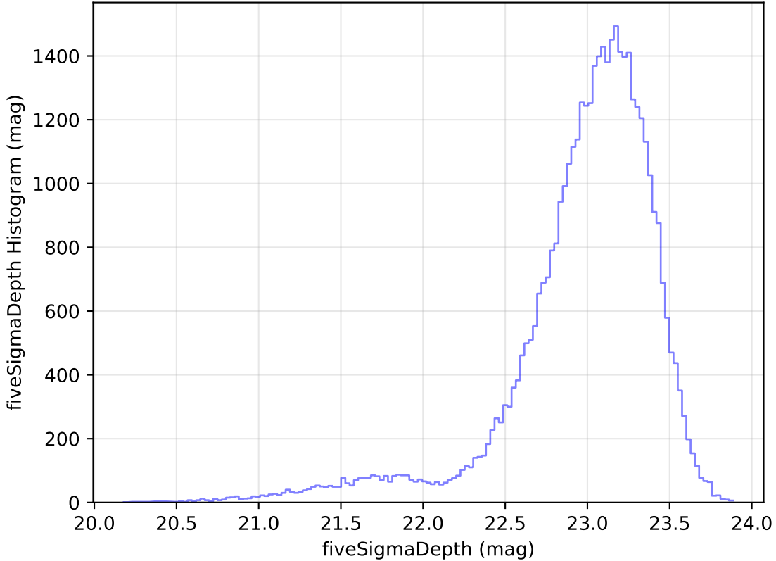
internal_u_expt45_nscale1.2v3.4_10yrs Yr 1 z band: fiveSigmaDepth Histogram
