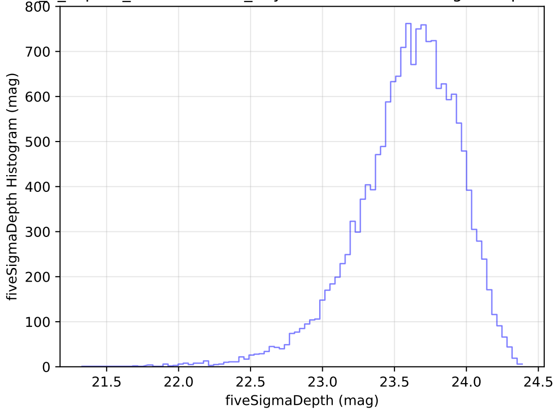
internal_u_expt45_nscale1.2v3.4_10yrs Yr 1 u band: fiveSigmaDepth Histogram
