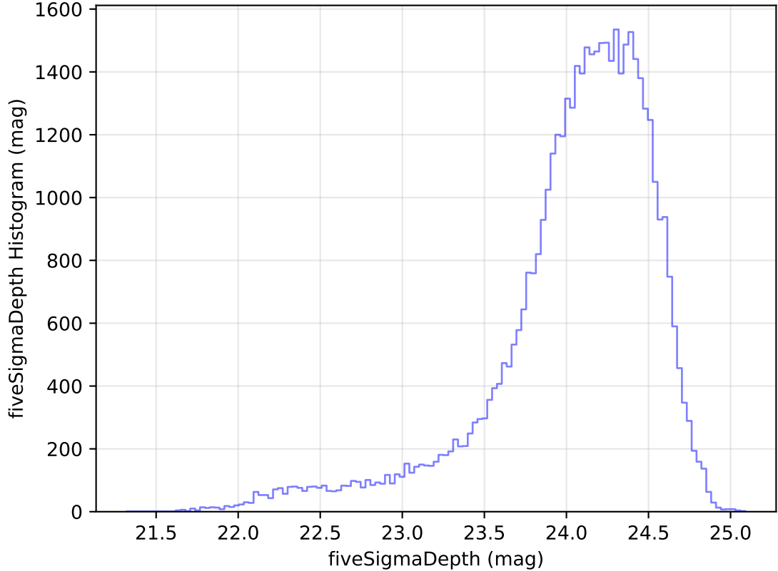
internal_u_expt45_nscale1.2v3.4_10yrs Yr 1 r band: fiveSigmaDepth Histogram
