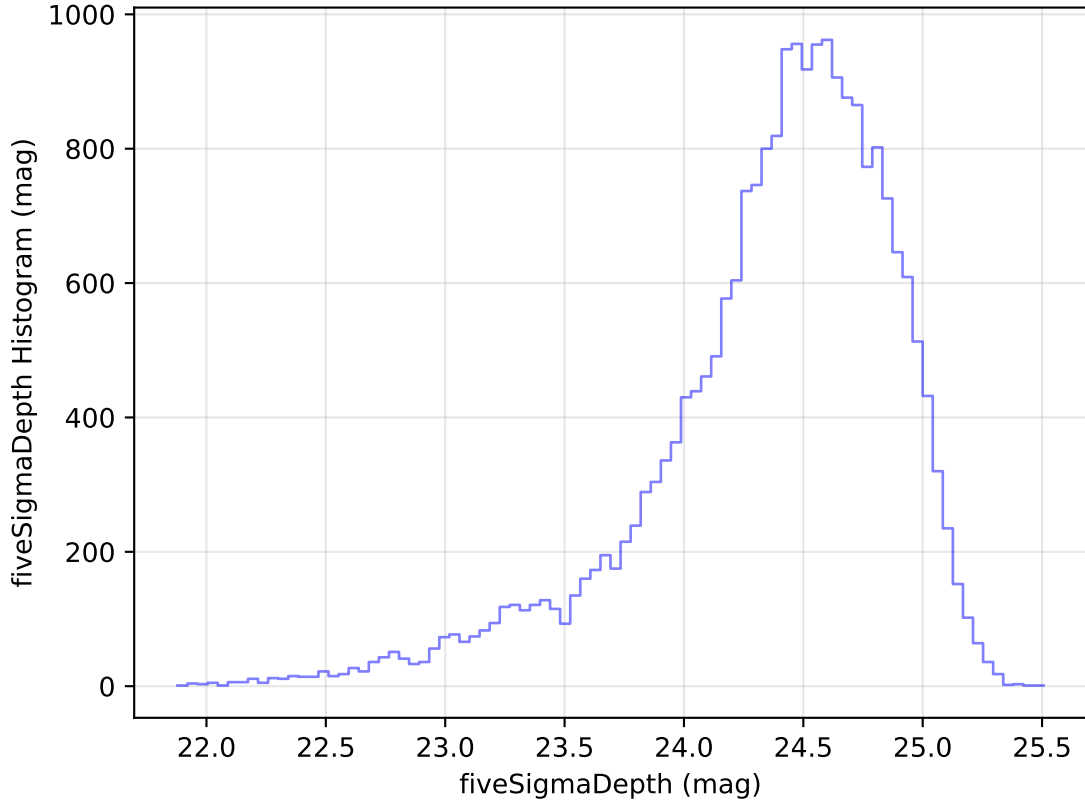
internal_u_expt45_nscale1.2v3.4_10yrs Yr 1 g band: fiveSigmaDepth Histogram
