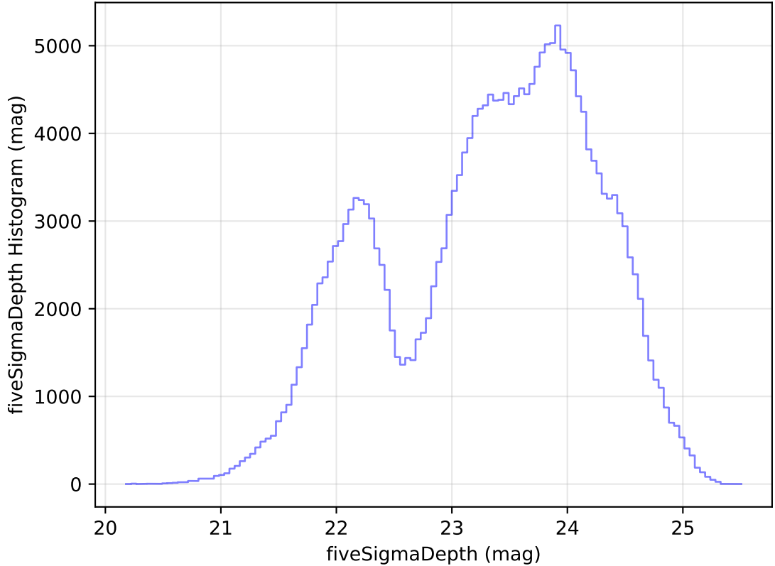
internal_u_expt45_nscale1.2v3.4_10yrs Yr 1 all bands: fiveSigmaDepth Histogram
