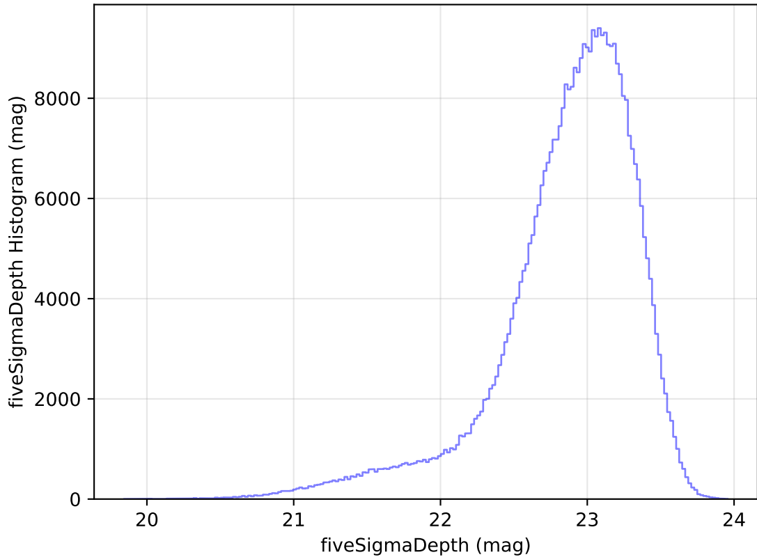
internal_u_expt45_nscale1.2v3.4_10yrs WFD z band: fiveSigmaDepth Histogram
