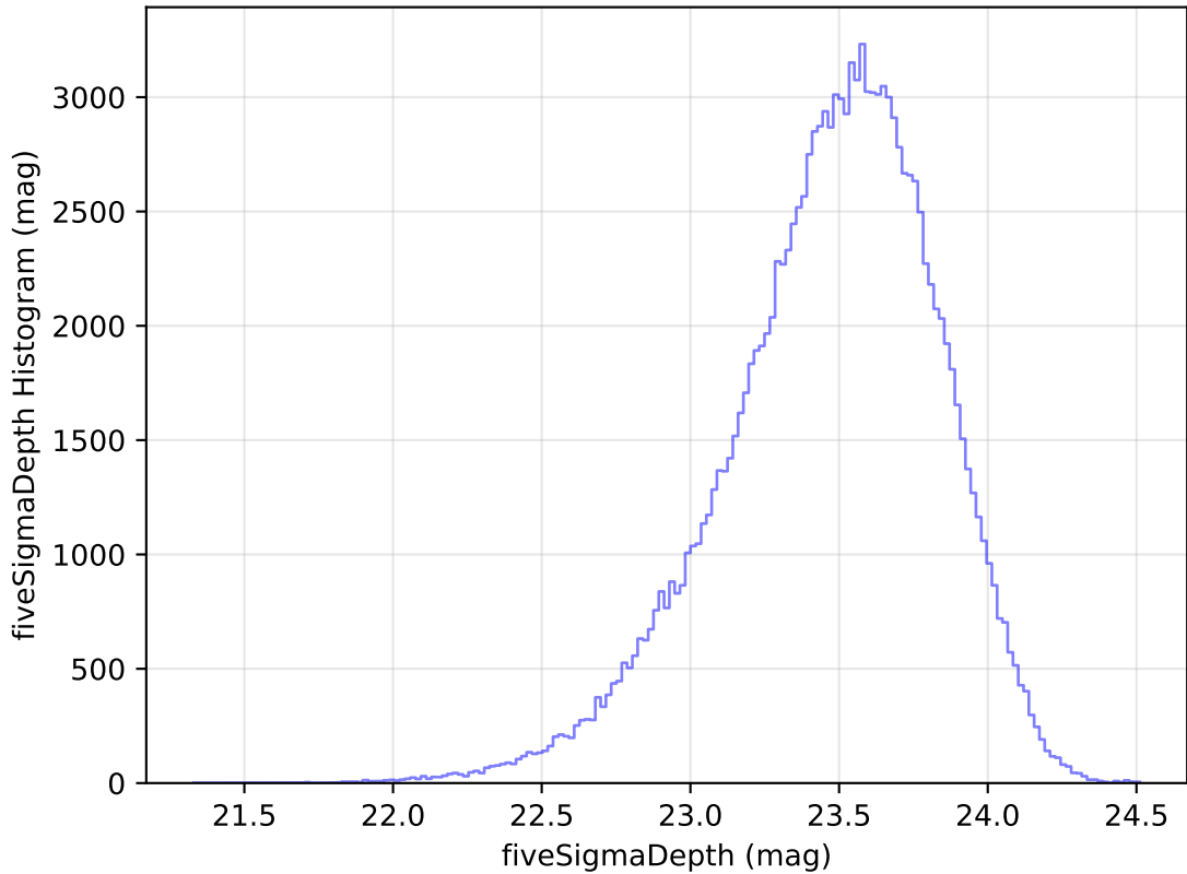
internal_u_expt45_nscale1.2v3.4_10yrs WFD u band: fiveSigmaDepth Histogram
