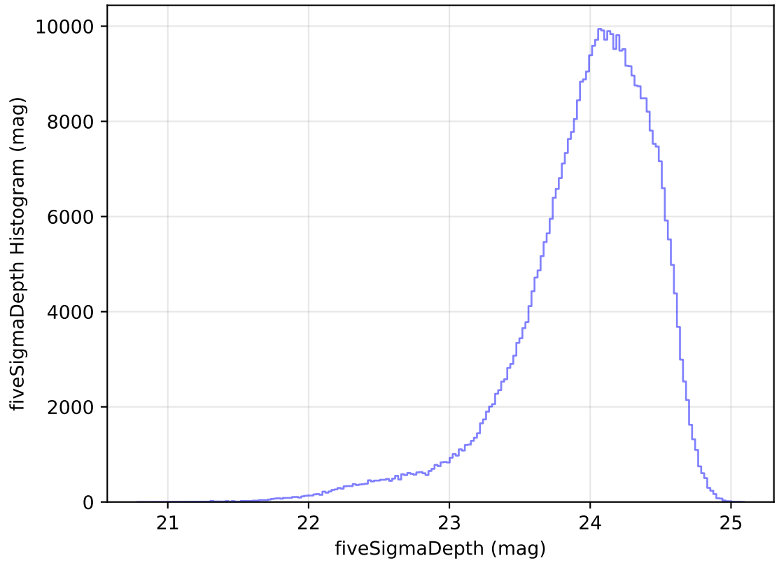
internal_u_expt45_nscale1.2v3.4_10yrs WFD r band: fiveSigmaDepth Histogram
